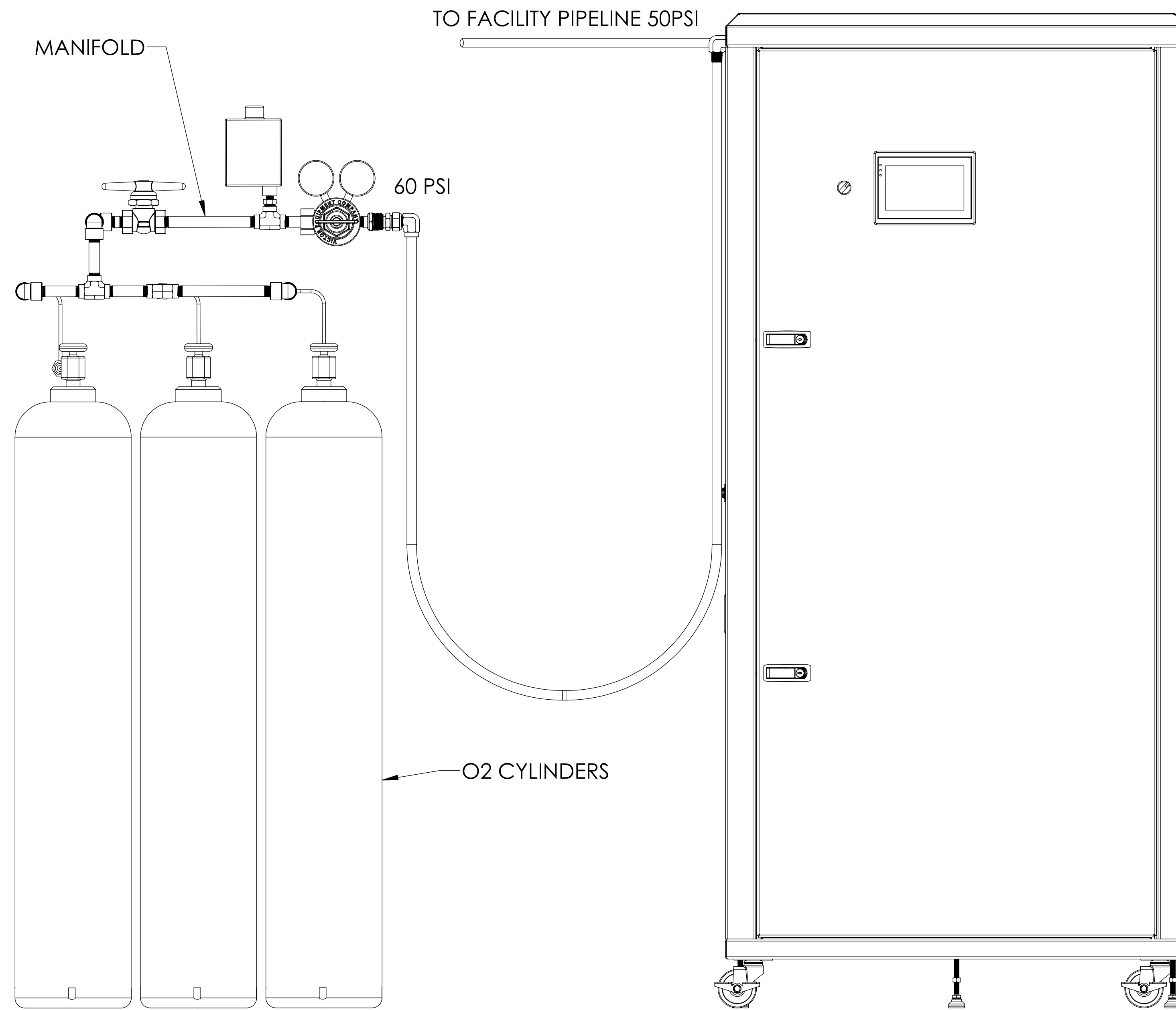
FRONT VIEW
