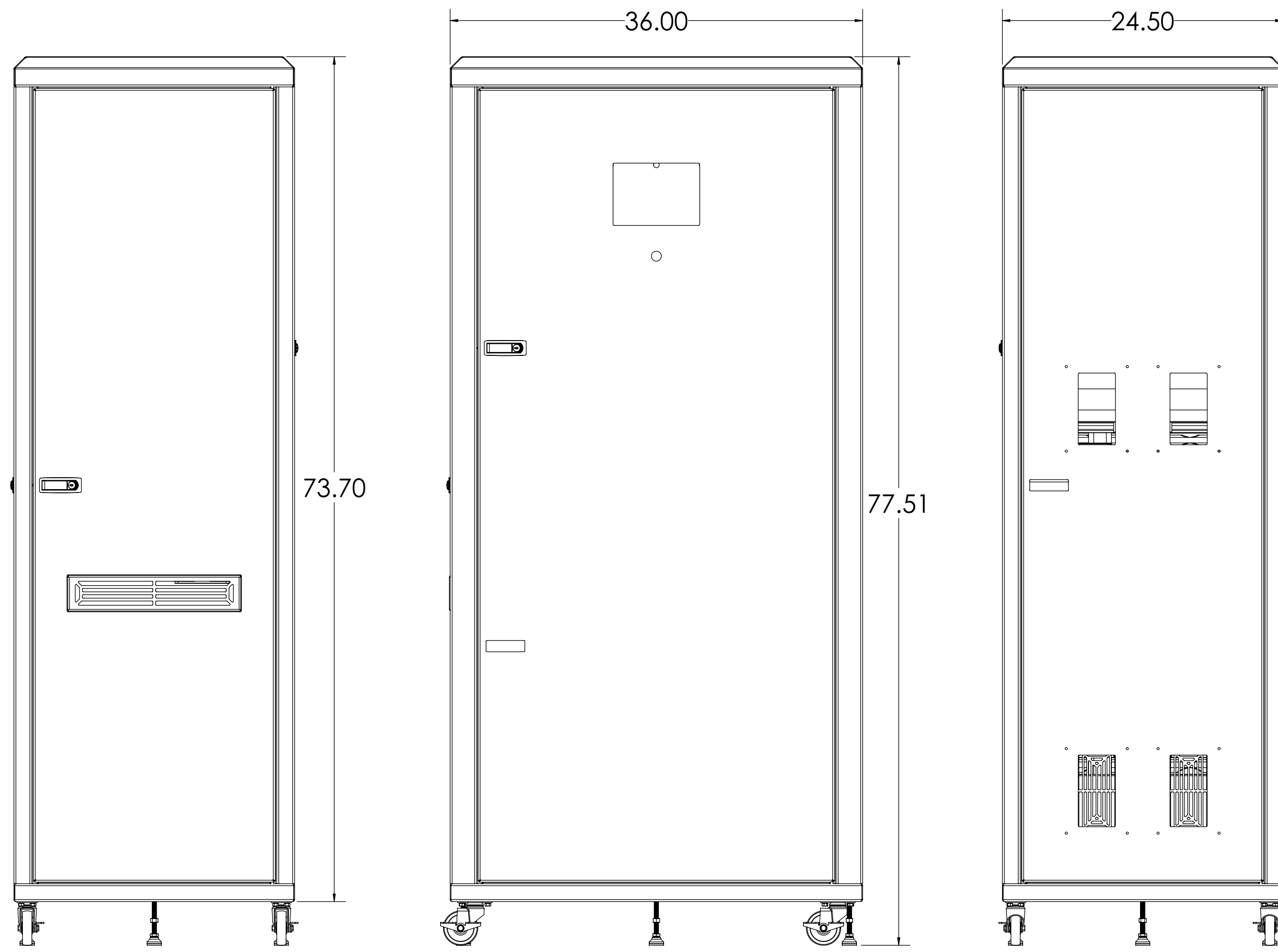
LEFT SIDE VIEW
